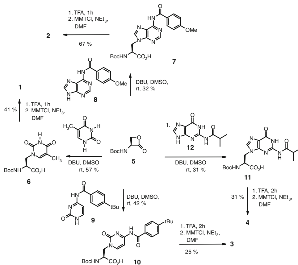
Scheme 1 Synthesis of Boc- and MMT-protected nucleoside amino acids with acyl protected nucleobases
